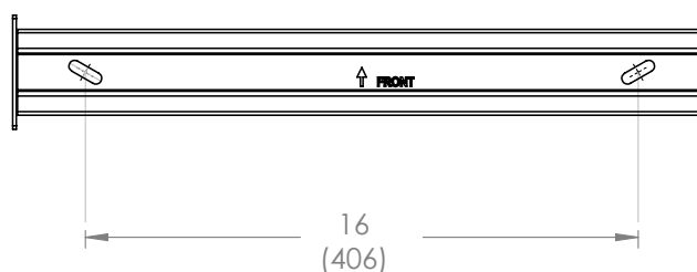
WALL PLATE MOUNTING HOLES
